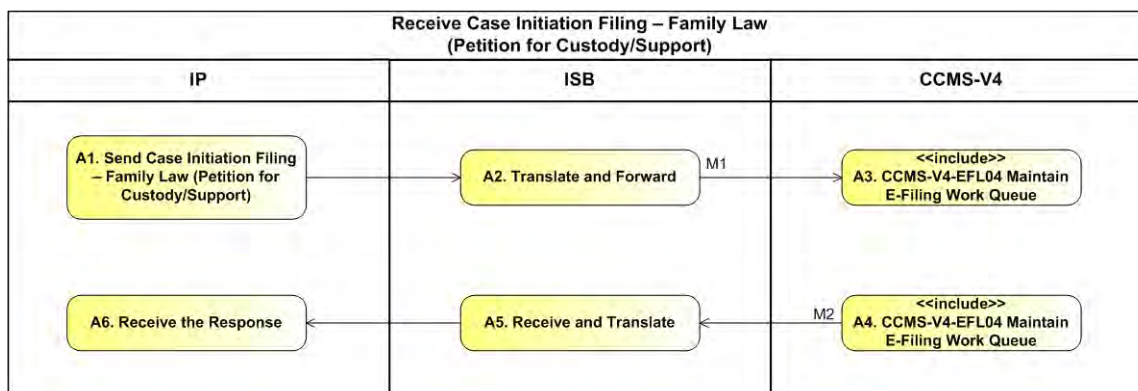
Figure 2: Receive Case Initiation Filing – Family Law (Petition for Custody/Support) Activity Diagram
